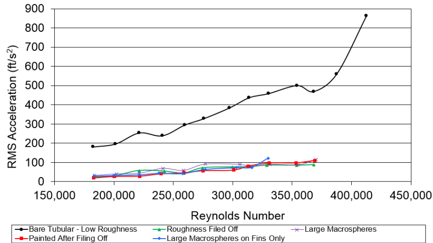
Figure 5 – Downstream Tubular Accelerations for Helical Strakes with Simulated Hard Growth
