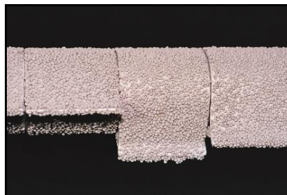
Figure 6 – Large Macrospheres on Fairings (Rough Fairings)
